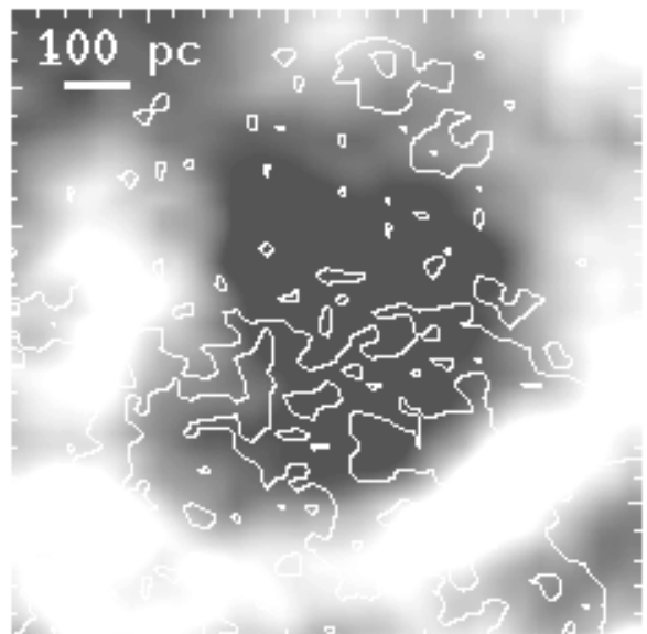
FIG. 17.—H I image of Holmberg II region 13 overplotted with the 21 and 21.7 mag \text{arcsec}^{-2} FUV surface brightness contours.
