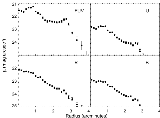
FIG. 4.—Optical and FUV surface brightness profiles of Holmberg II
