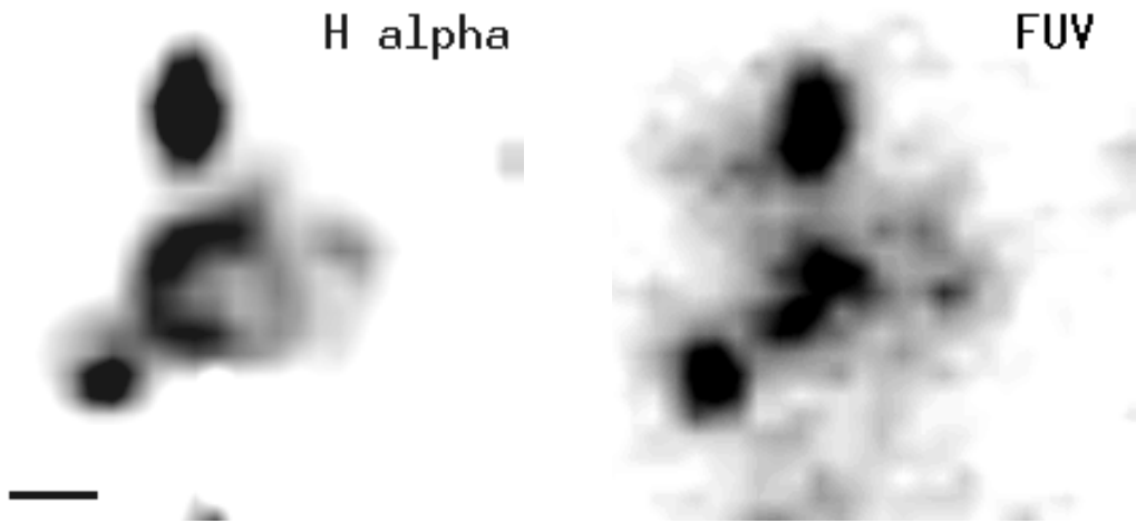
FIG. 9.—Registered H \alpha and FUV images of Holmberg II, region 6. The dark bar in the lower left-hand corner represents 100 pc in Figs. 9, 10, 12, and 13.
