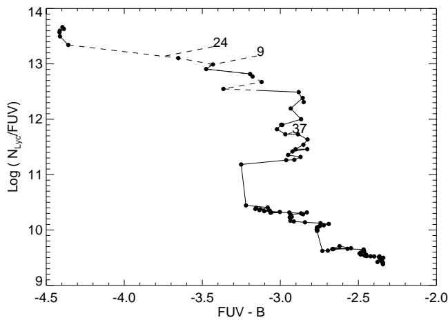
FIG. 7.—Cluster model with three Holmberg II data points. The uncorrected data points are represented by the region number. The age groups are shown by the alternating dotted and solid lines of the model: group 1 (first dotted line) = 0–3.5 Myr, group 2 (first solid line) = 3.5–4.5 Myr, group 3 (next dotted line) = 4.5–6.3 Myr; group 4 (last solid line) \geq 6.3 Myr.
