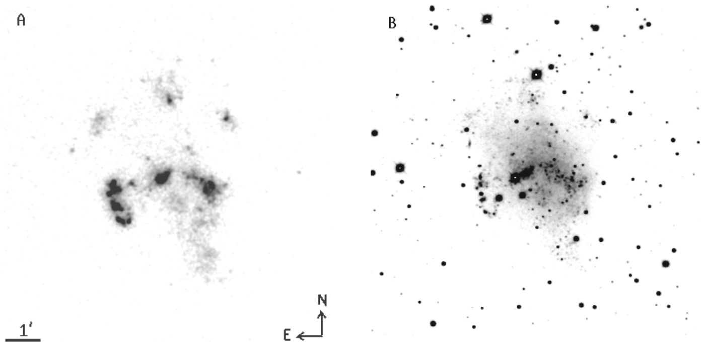
FIG. 1.—(a) Registered FUV and (b) R -band images of Holmberg II
