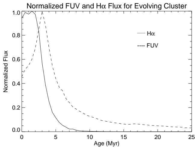
FIG. 11.—Normalized FUV and H\alpha flux for an evolving star cluster
