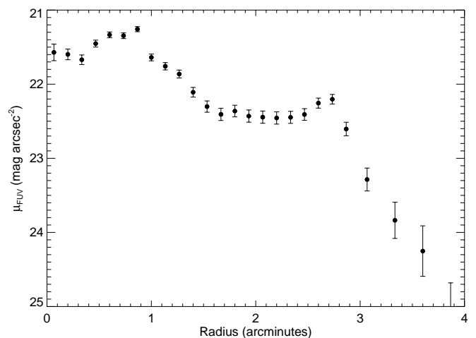
FIG. 3.—FUV surface brightness profile of Holmberg II
