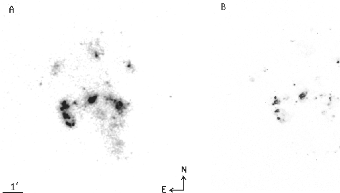
FIG. 5.—(a) Registered FUV and (b) H\alpha images of Holmberg II
