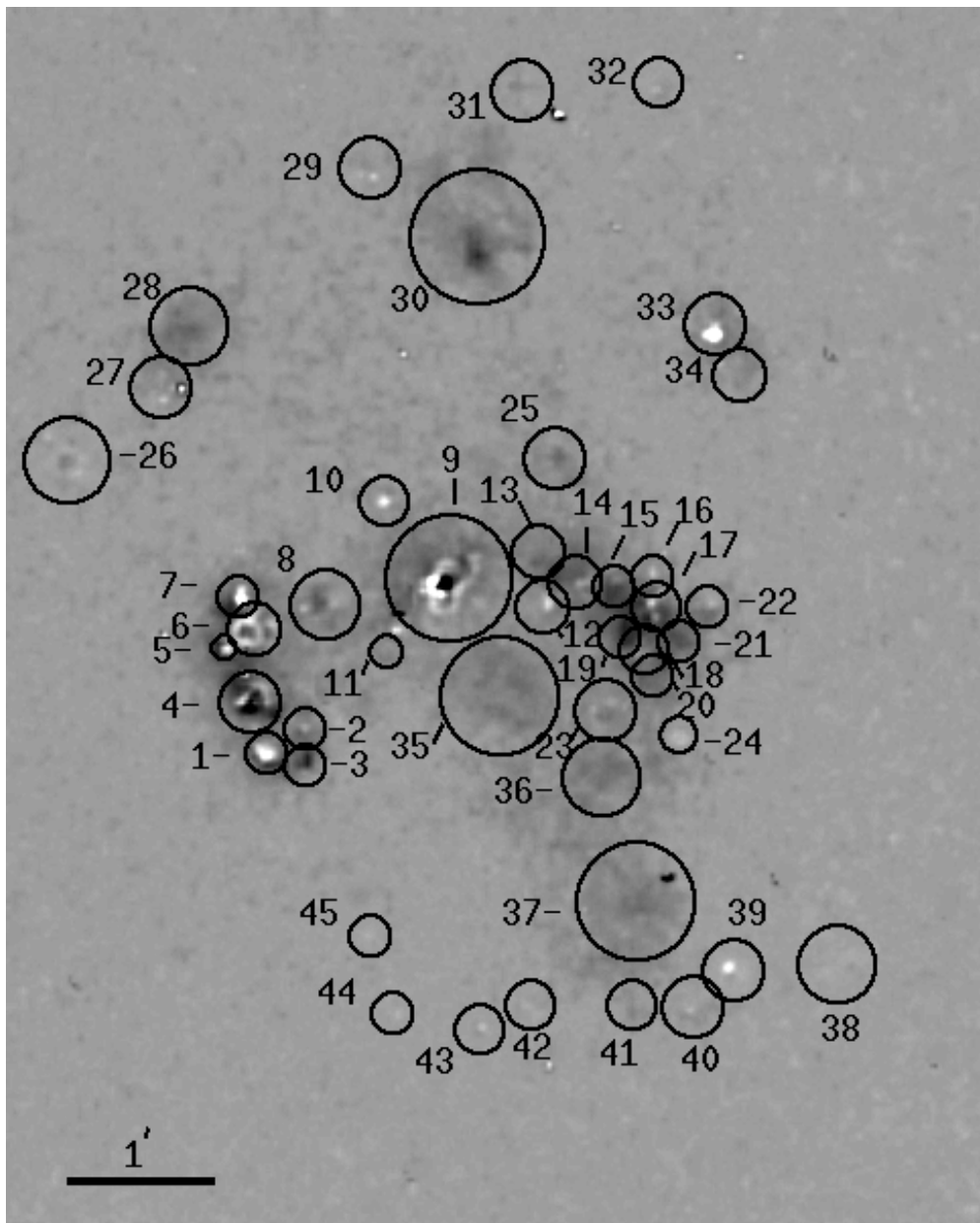
FIG. 6.—Holmberg II star formation regions on an FUV, H\alpha difference image; areas with H\alpha and no FUV emission are white and areas with FUV and no H\alpha emission are black.
