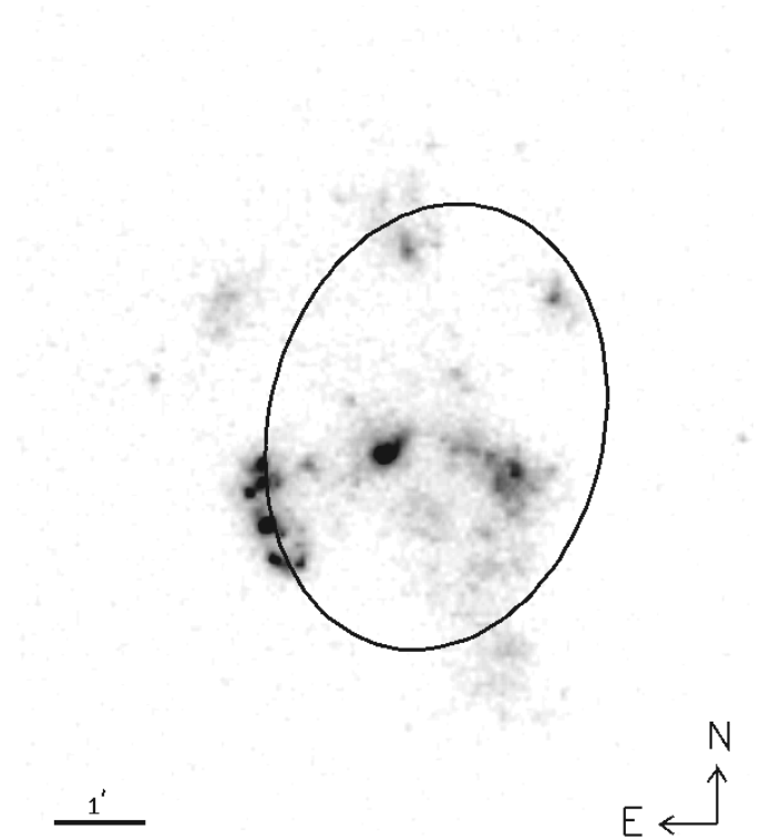
FIG. 20.—H I image of Holmberg II shown with a 2' ellipse. The interior of the ellipse represents the solid body regime of the neutral gas disk.
