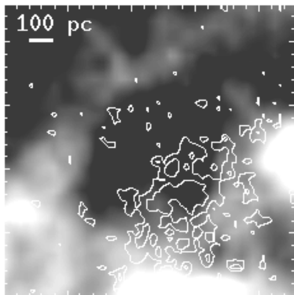
FIG. 16.—H I image of Holmberg II region 28 overplotted with the 21.5 and 22 mag \text{arcsec}^{-2} FUV surface brightness contours. Figs. 16, 17, and 18 are displayed so that the H I holes appear as dark voids and the H I density enhancements are bright.
