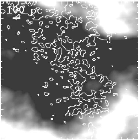
FIG. 18.—H I image of Holmberg II regions 36 and 37 overlaid with the 19, 20.5, and 21.75 mag arcsec -2 FUV surface brightness contours.
