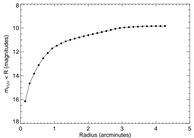
FIG. 2.—FUV growth curve of Holmberg II
